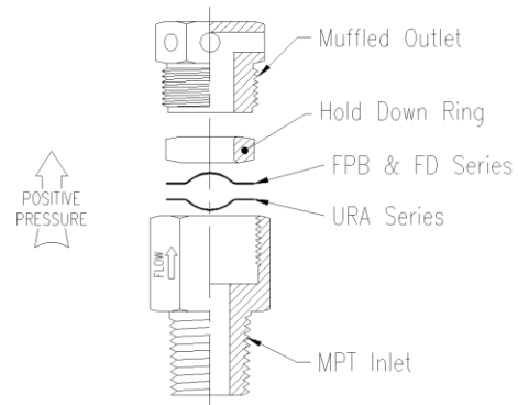
Figure 4 – Flat Seated Disk Screw Type Holder
