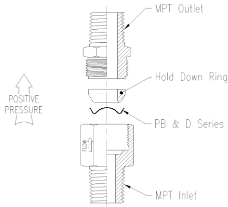
Figure 3 – Angle Seated Disk Screw Type Holder
